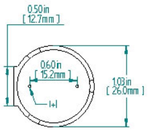
REAR
