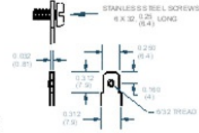
"S" TERMINALS
